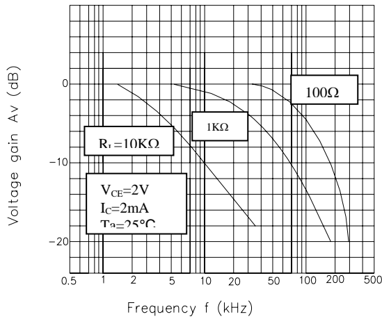
Fig.11 Frequency Response
